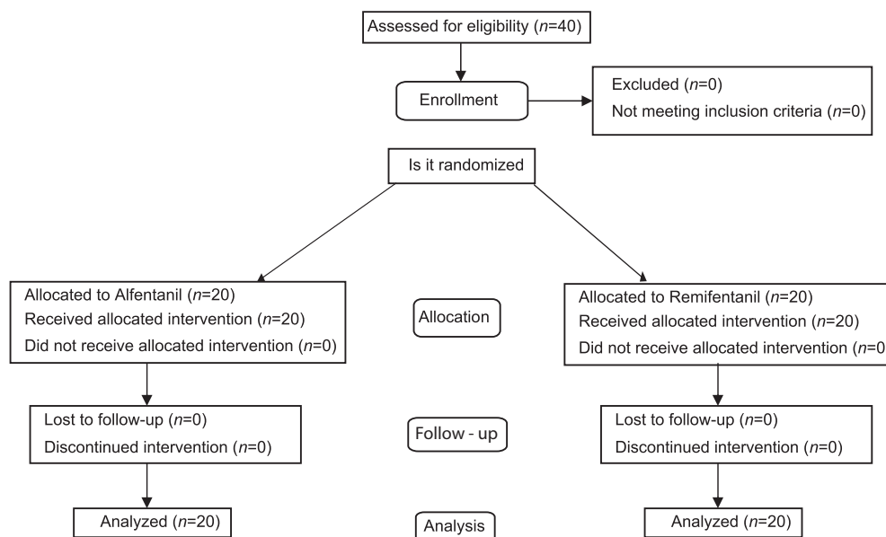
Figure 1: Methodology flowchart
