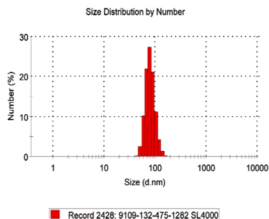
Figure 2. Size distribution of nanosilver particles in SilvoSept®.
