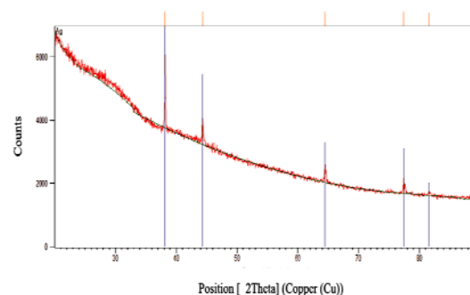
Figure 1. X-ray diffraction pattern of Ag nanoparticles.
