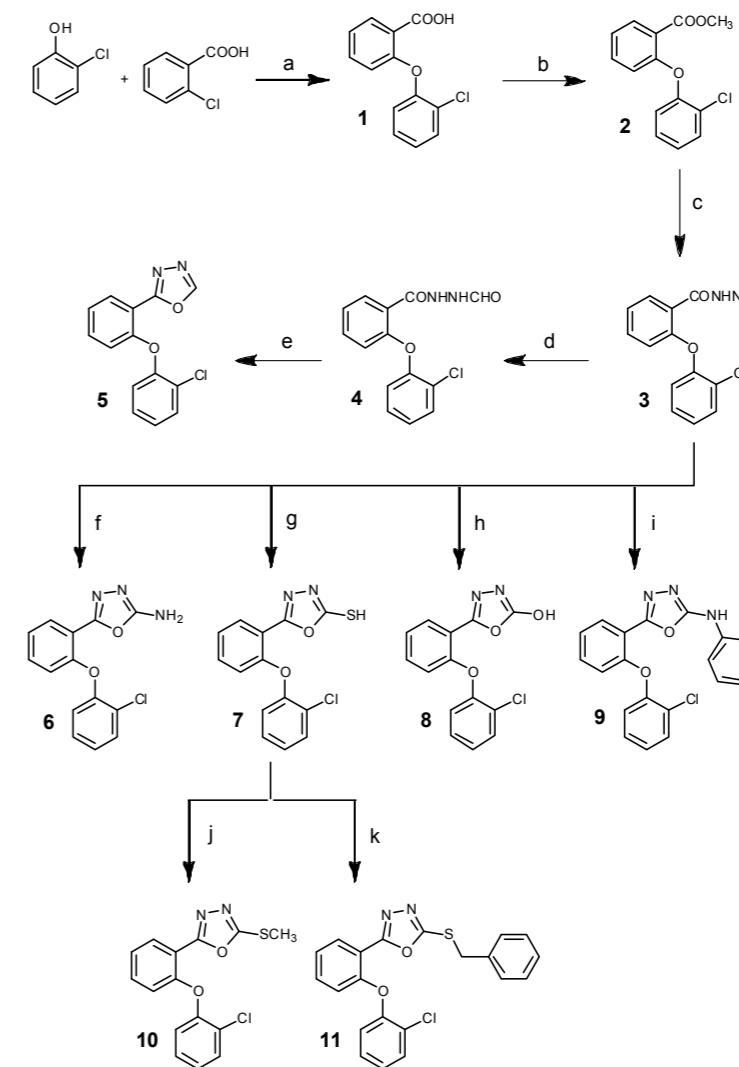
Figure 2. Reagents: (a) 1) Na, dry methanol, rt, 2h; 2) DMF, Cu, reflux; (b) methanol, H 2 SO 4 , reflux, 7 h; (c) methanol, NH 2 NH 2 .H 2 O, stir, rt, 12 h; (d) formic acid, reflux, 4 h; (e) P 2 O 5 , xylene, reflux, 3 h; (f) BrCN, dioxan, stir, rt, overnight; (g) CS 2 , ethanol, KOH, reflux, 7 h; (h) 1,1'-carbonyldiimidazole, triethylamine, dry THF, 0°C, 5h then rt, overnight; (i) toluene, phenylisocyanate, DCC, reflux, 7 h; (j) methyl iodide, ethanol, NaOH, ultrasonication, 5 min; (k) benzyl chloride, ethanol, NaOH, ultrasonication, 5 min.
