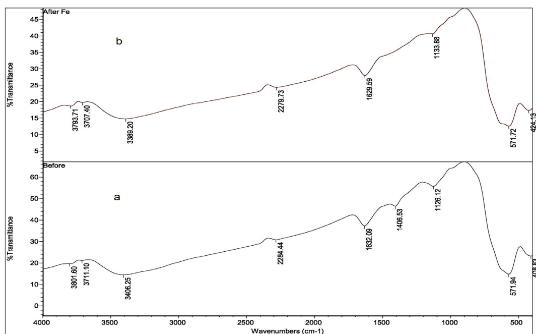
Fig. 3. FTIR spectra of the iron oxide before (a) and after (b) Fe ions loaded on magnetic iron oxide nanoparticles.
