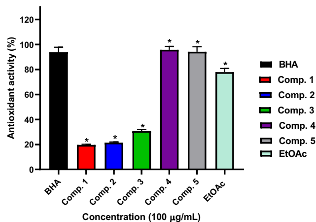
Fig. 3. Antioxidant activity of isolated compounds ( 1–5 ) and EtOAc extract of C. italica by DPPH method. * Compared to BHA (Positive control); (one-way ANOVA followed by Tukey Kramer). Data are the mean \pm SE. ( n = 3 ).
