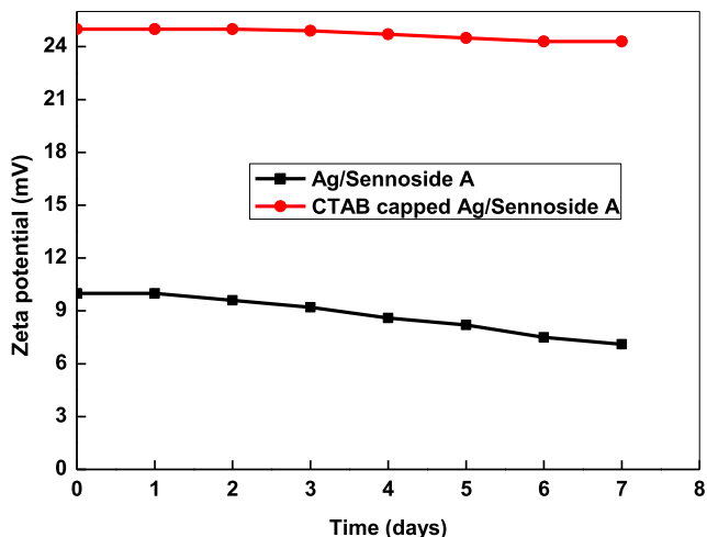
Fig. 5. Zeta potentials as a function of time for the Ag/Sennoside A and CTAB capped Ag/Sennoside A NPs. (Particle charge was negative for both samples).
