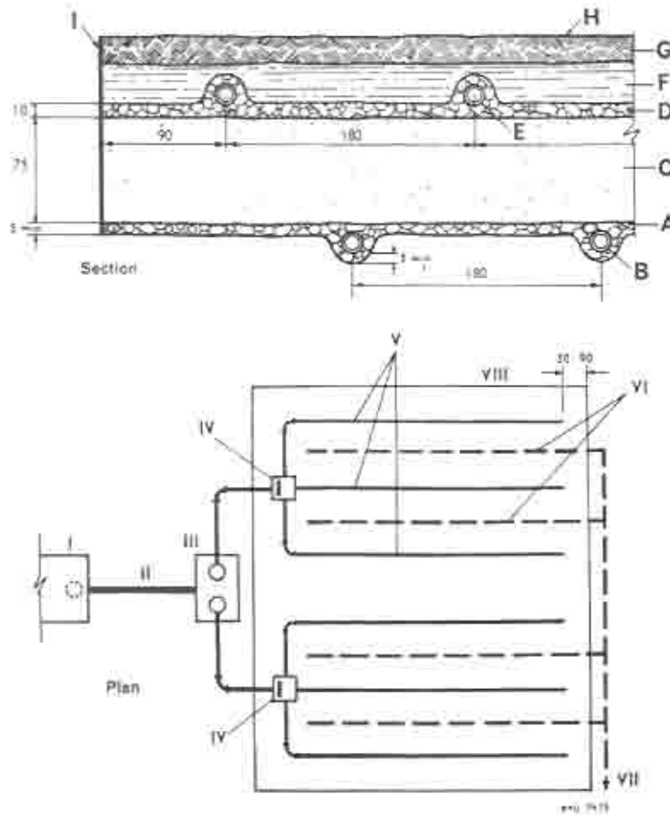
Fig. 53. SUBSURFACE SAND FILTER
