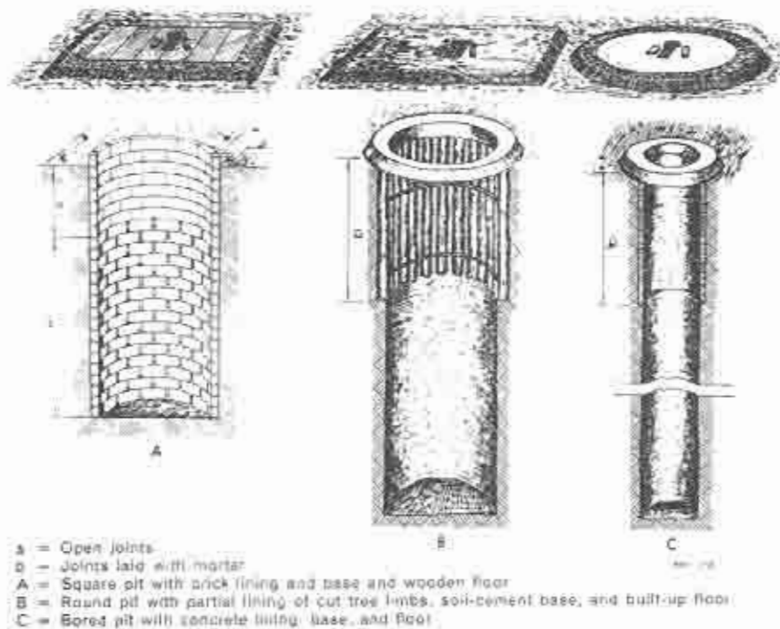
Fig.13. VARIOUS COMBINATIONS OF DIFFERENT TYPES OF PIT, PIT LINING, BASE AND FLOOR
