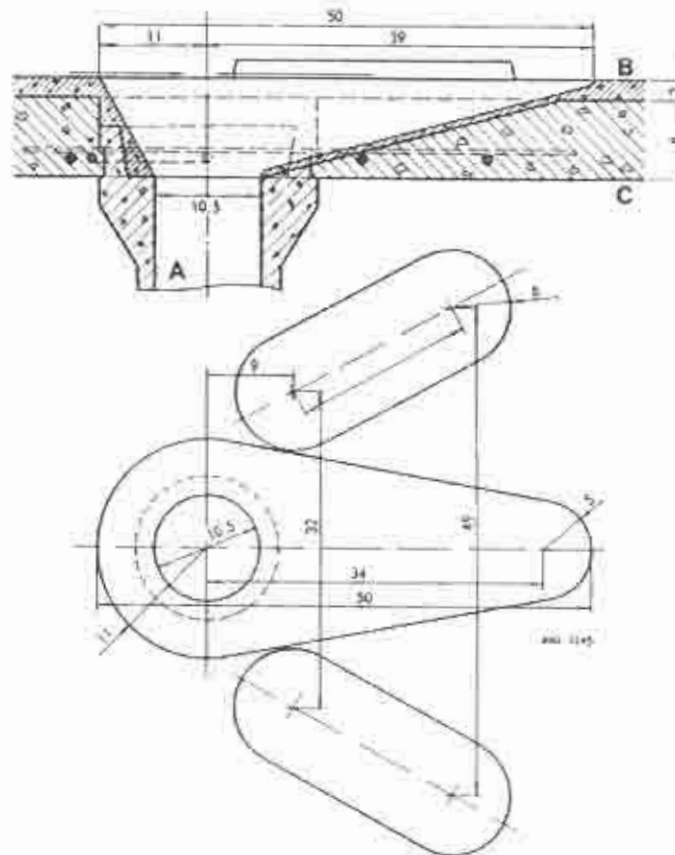
Fig. 41 BOWL FOR PUBLIC AQUA PRIVY
