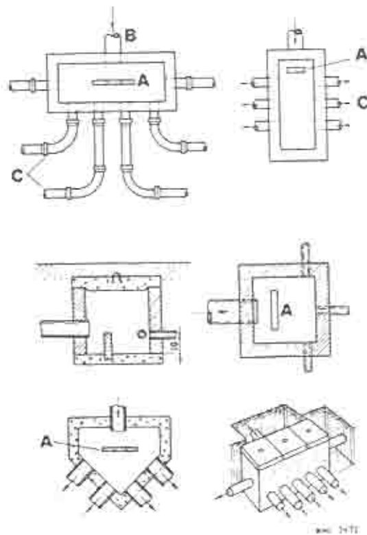
Fig. 51. TYPES OF DISTRIBUTION BOX
