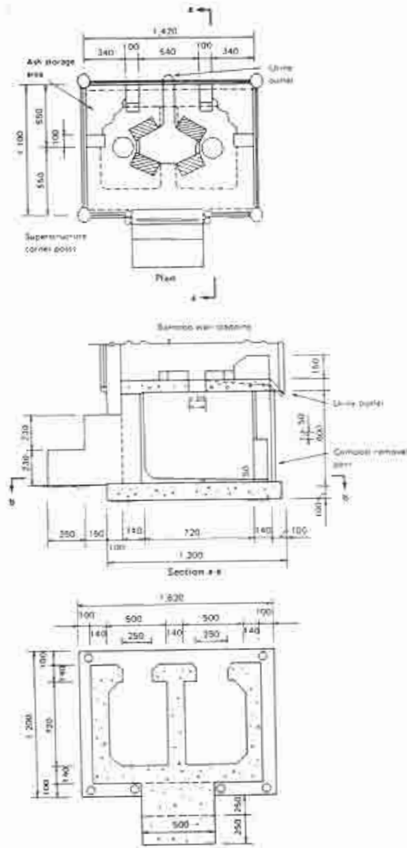
Fig. 33. DOUBLE-VAULT COMPOSTING LATRINE USED IN VIETNAM
