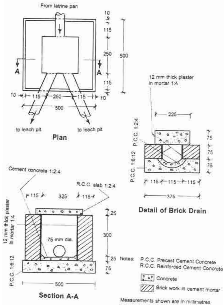
Fig. 36. DETAILS OF DRAIN AND JUNCTION CHAMBER
