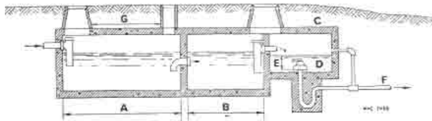
Fig. 48. SEPTIC TANK WITH TWO COMPARTMENTS AND DOSING CHAMBER
