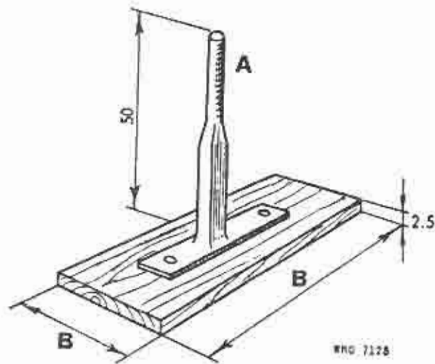
Fig. 6. SIMPLE HOLE COVER
