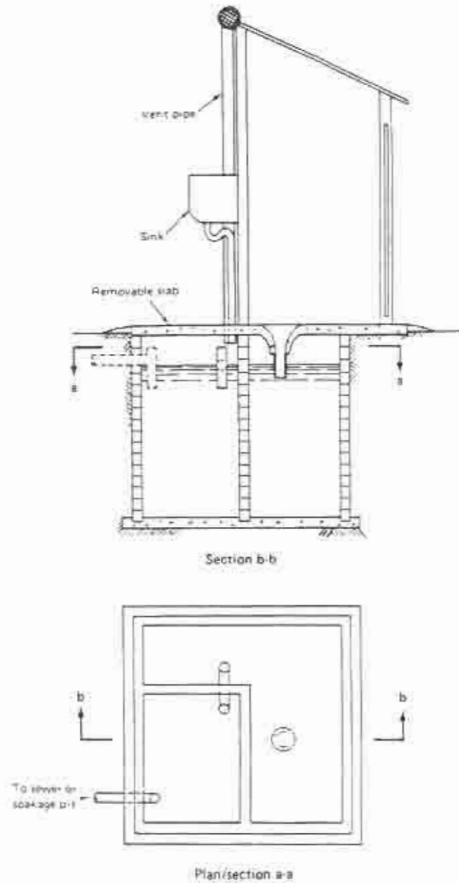
Fig. 43. IMPROVED SEWERED AQUA PRIVY WITH SULLAGE DISPOSAL
