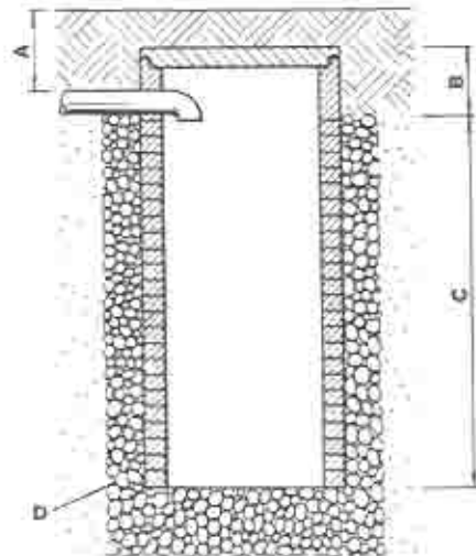
Fig. 49. SEEPAGE PIT
