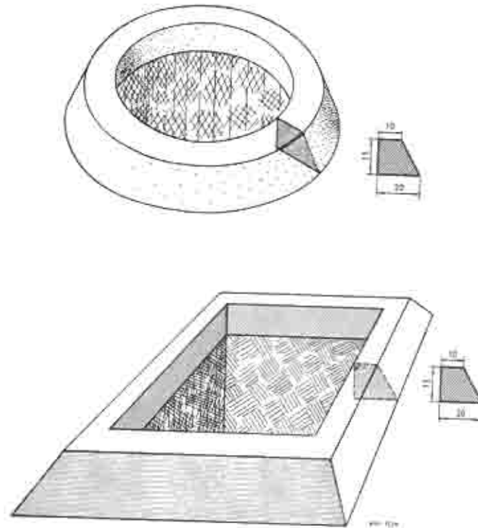
Fig. 15. CEMENT BASE
