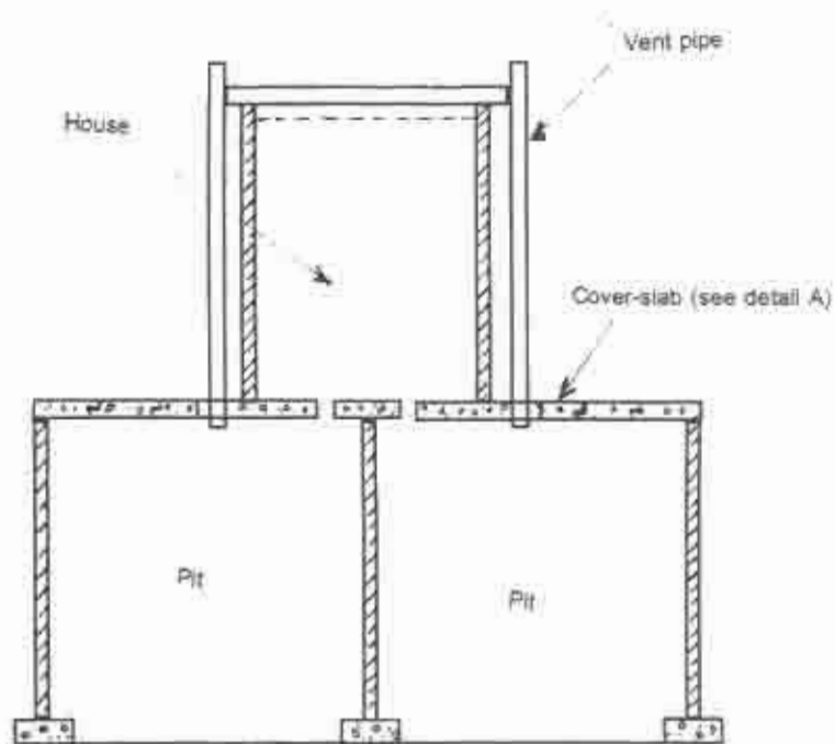
Fig. 29. COVER SLAB DETAILS FOR ALTERNATING TWIN-PIT VIP LATRINES
