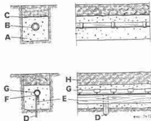
Fig. 50. ABSORPTION TRENCHES
