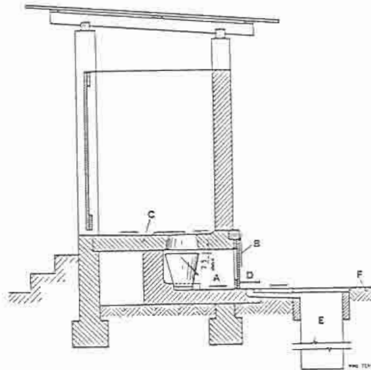
Fig. 60. THE BUCKET LATRINE
