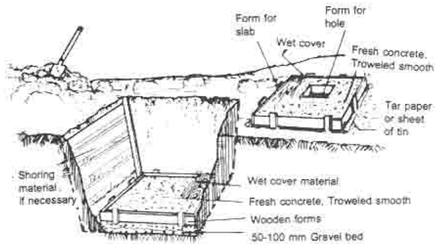
Fig. 44. CONSTRUCTION DETAILS FOR AQUA PRIVY
