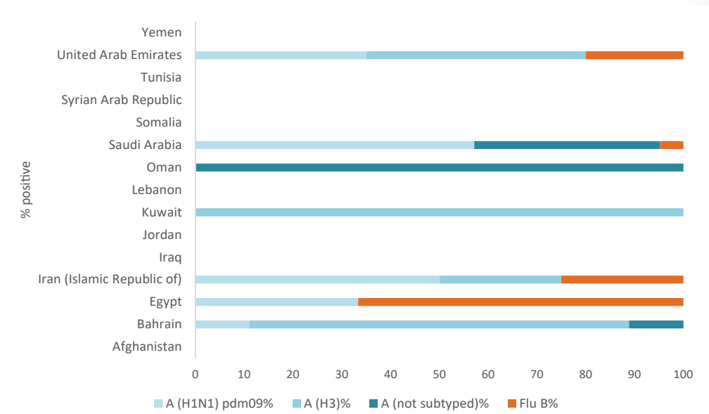
Figure 3. Percentage of influenza virus types and subtypes by country, week 34, 2025
