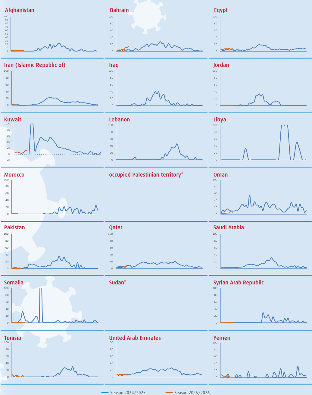
Figure 4. Percent positivity trends among EMR member states for two seasons: from week 27, 2024 till week 26, 2025 and from week 27, 2025 till week 34, 2025
