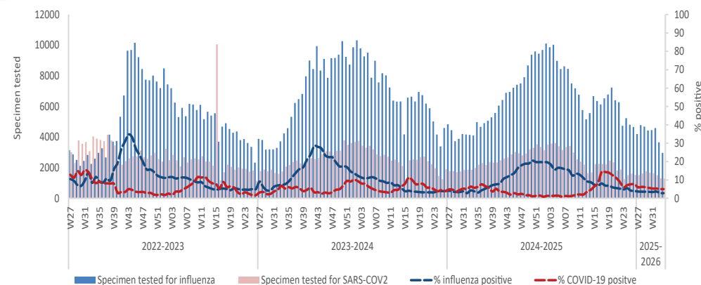
Figure 1. Influenza and SARS-CoV-2 tested specimens and percent positivity in the Region from week 27, 2022 to week 34, 2025
