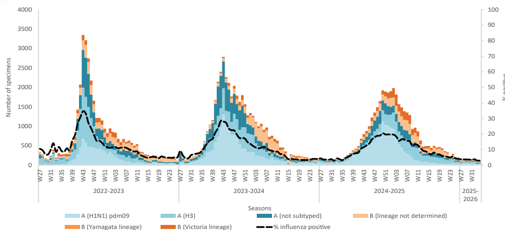
Figure 2. Number of specimens by influenza virus subtypes/lineages and percentage of specimens testing positive for influenza viruses in the Region from week 27, 2022 to week 34, 2025
