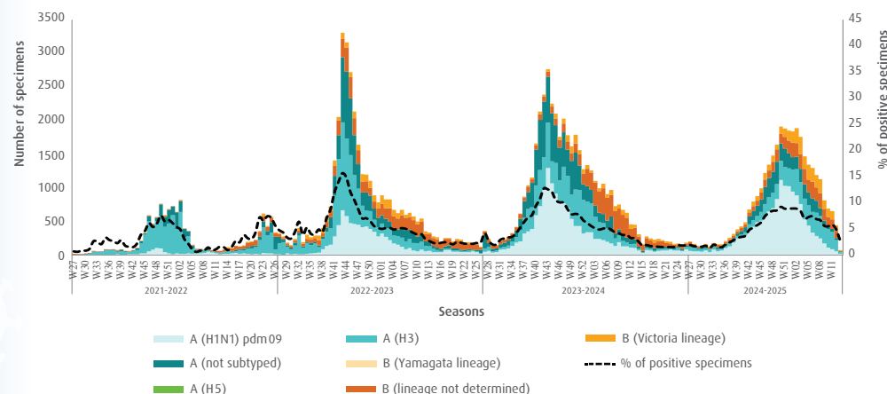
Figure 2. Number of specimens by influenza virus subtypes/lineages and percentage of specimens testing positive for influenza viruses in the Region from week 27, 2021 to week 13, 2025
