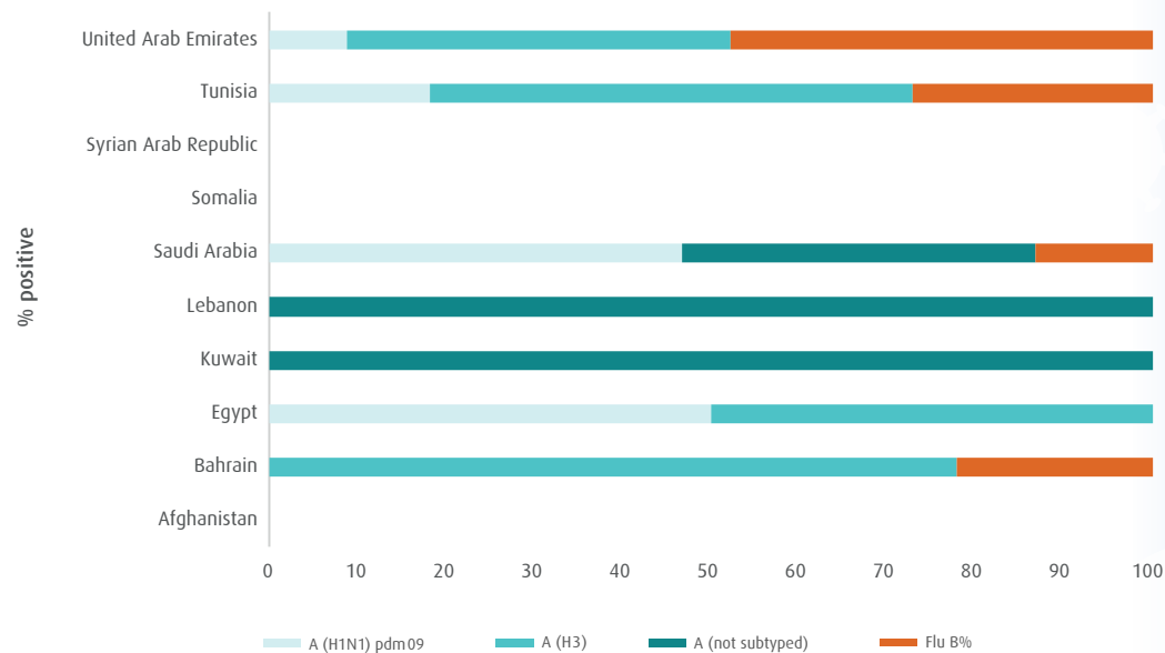
Figure 3. Percentage of influenza virus types and subtypes by country, week 13, 2025
