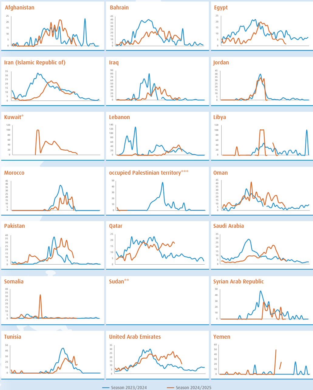
Figure 4. Percent positivity trends among EMR member states for two seasons: from week 27, 2023 till week 26, 2024 and from week 27, 2024 till week 13, 2025
