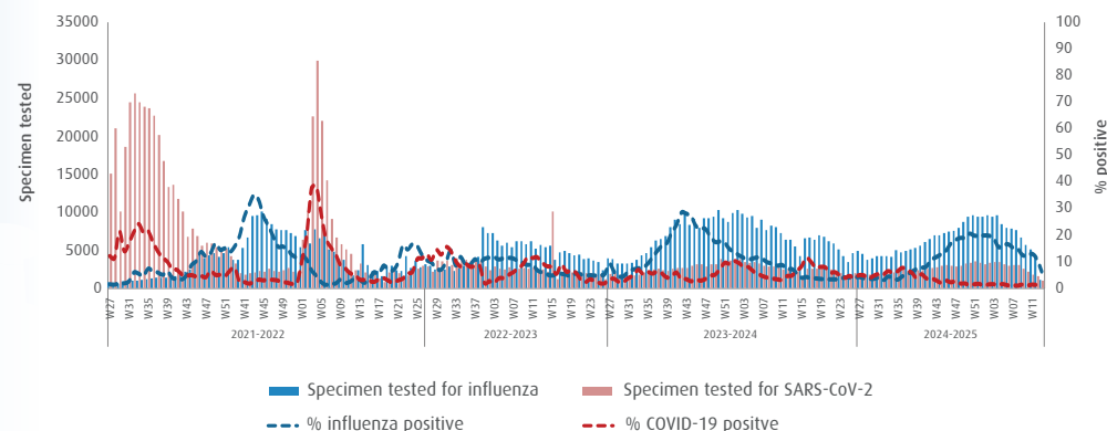
Figure 1. Influenza and SARS-CoV-2 tested specimens and percent positivity in the Region from week 27, 2021 to week 13, 2025
