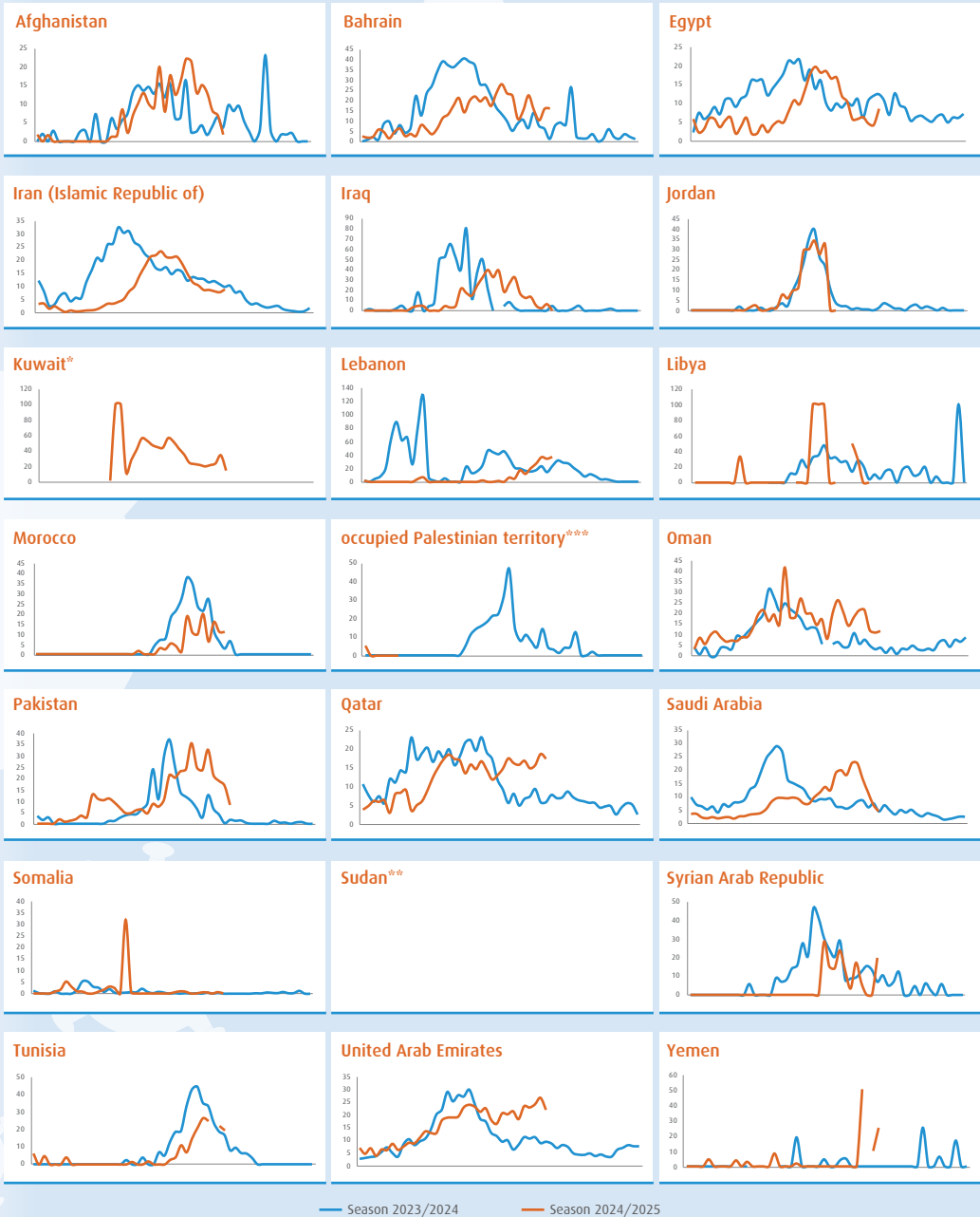
Figure 4. Percent positivity trends among EMR member states for two seasons: from week 27, 2023 till week 26, 2024 and from week 27, 2024 till week 10, 2025
