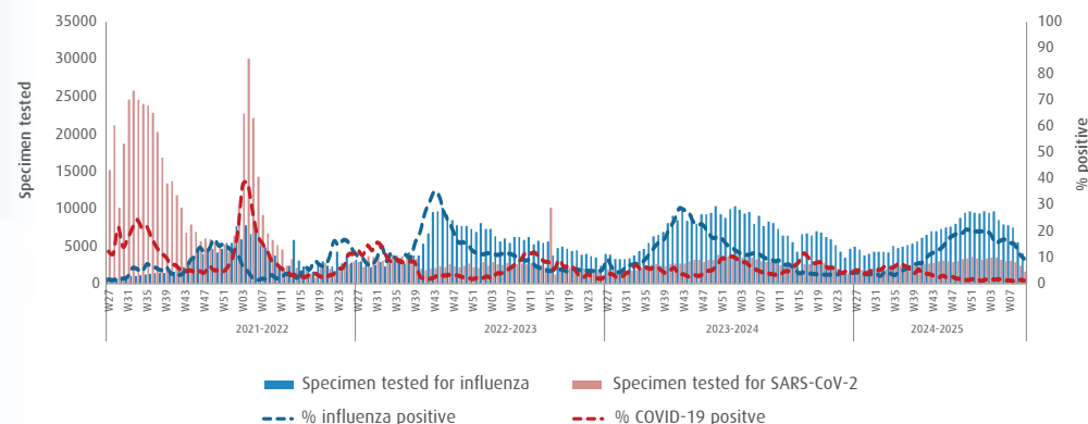
Figure 1. Influenza and SARS-CoV-2 tested specimens and percent positivity in the Region from week 27, 2021 to week 10, 2025
