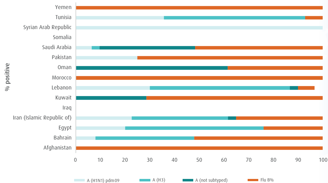
Figure 3. Percentage of influenza virus types and subtypes by country, week 10, 2025
