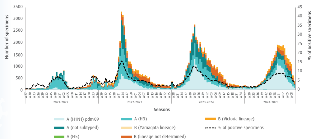
Figure 2. Number of specimens by influenza virus subtypes/lineages and percentage of specimens testing positive for influenza viruses in the Region from week 27, 2021 to week 10, 2025
