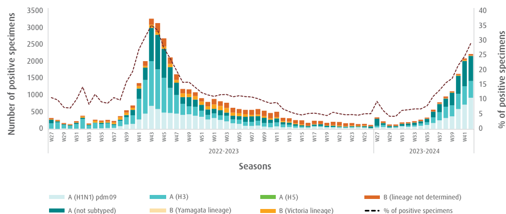
Fig. 3. Proportion of influenza subtypes/lineages in the Region, week 42, 2023
