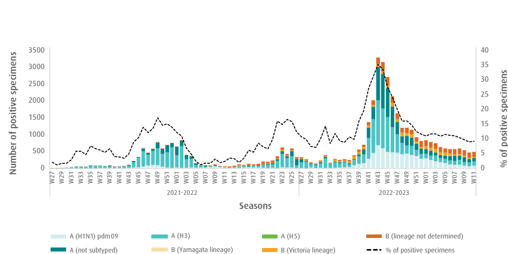
Fig. 2. Number of positive specimens by subtype/lineage and percentage of specimens testing positive for influenza viruses starting from week 27, 2021 till week 11, 2023
