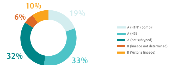
Fig. 3. Proportion of influenza subtypes/lineages in the Region, week 47, 2022
