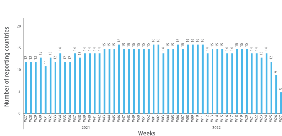
Fig. 1. Number of reporting countries to EMFLU/FluNet by week in the Region, week 27, 2021 – week 27, 2022
