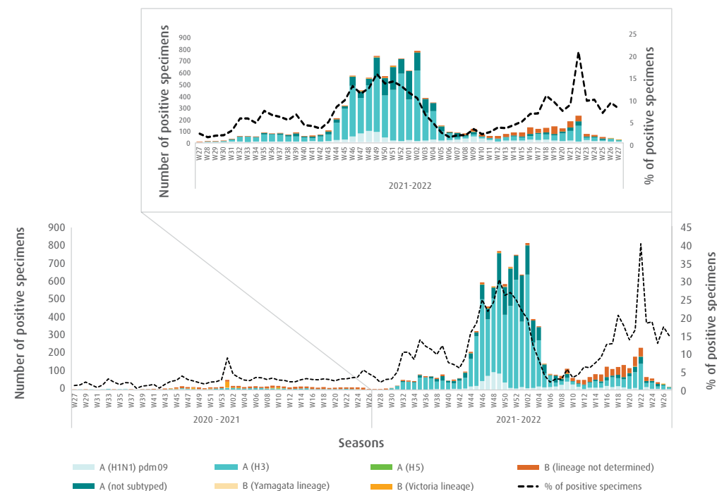
Fig. 3. Proportion of influenza subtypes/lineages in the Region, week 27, 2022
