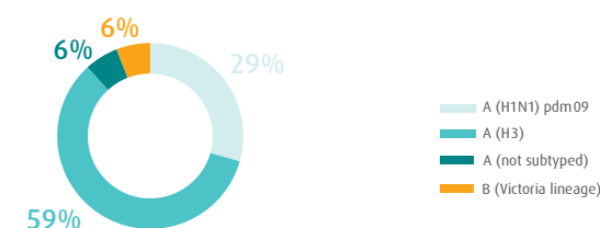
Fig. 3. Proportion of influenza subtypes/lineages in the Region, week 27, 2022
