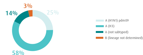
Fig. 3. Proportion of influenza subtypes/lineages in the Region, week 4, 2022
