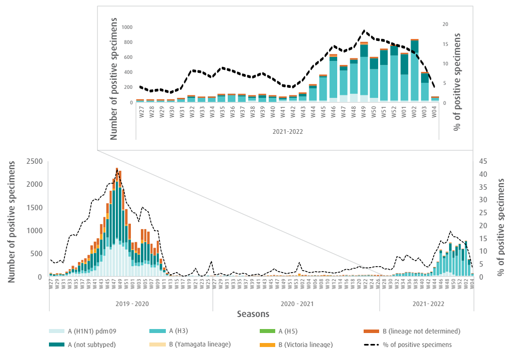
Fig. 3. Proportion of influenza subtypes/lineages in the Region, week 4, 2022
