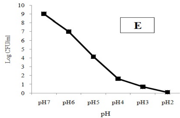
Figure 1. Viability curves of L. monocytogenes PTCC1297 exposed to different degrees of stresses (A) Heat, (B) Ethanol, (C) NaCl, (D) H 2 O 2 , (E) HCl incubation was performed in 250 mL-Erlenmeyer flasks containing 50 mL of listeria enrichment broth on a rotary shaker 150 rpm at 30°C for 24. Survivor plots (log 10 CFU/mL) were determined for each range of environmental conditions on listeria selective oxford agar
