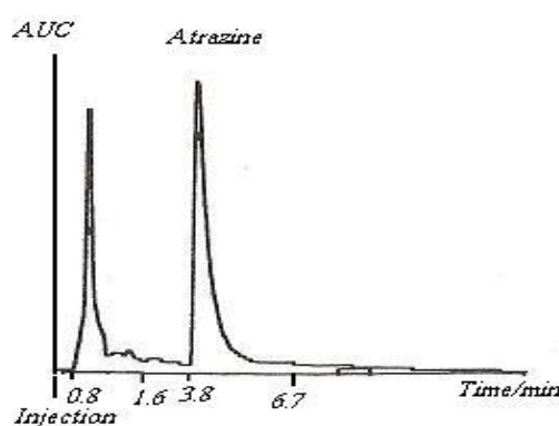
Fig. 5: The HPLC chromatogram of standard spiked atrazine at the concentration of 10 ppm before extraction. AUC: Area Under Curve
