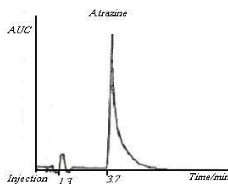
Fig. 6: The HPLC chromatogram of standard spiked atrazine at the concentration of 10 ppm after extraction. AUC: Area Under Curve
