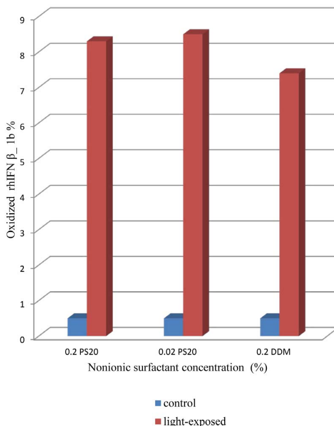
Figure 5. Oxidized rhIFN \beta_1b detected by RP-HPLC analysis. Formulations containing either 0.2% PS 20 or 0.02% PS20 or 0.2% DDM, respectively.
