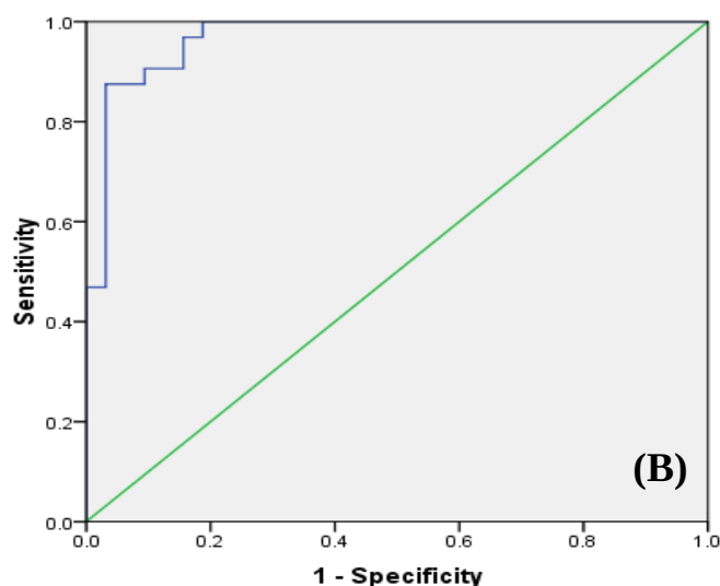
Fig. 4. ROC curve analysis. ROC curve shows AUCs of miR-21 and miR-221 (A) as well as the combination of two miRs (B). The green and blue lines represent miR-21 and miR-221, respectively.
