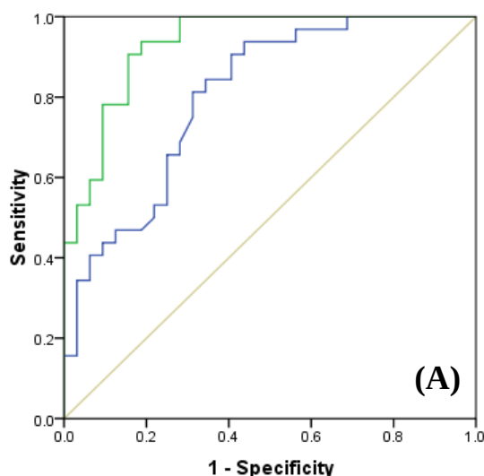
Fig. 4. ROC curve analysis. ROC curve shows AUCs of miR-21 and miR-221 (A) as well as the combination of two miRs (B). The green and blue lines represent miR-21 and miR-221, respectively.
