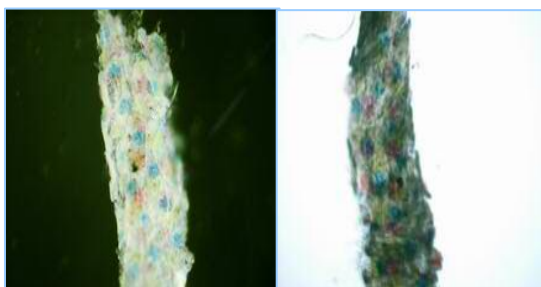
Figure 3: semi digested prey items were vomited by M. leidyi
