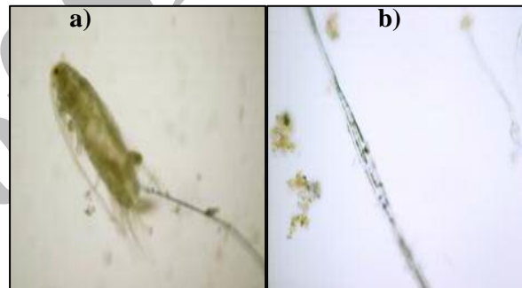
Figure 4: prey items in M. leidyi gut (a: Copepod ( Eurytemora grimmeri ), b: Algae)
